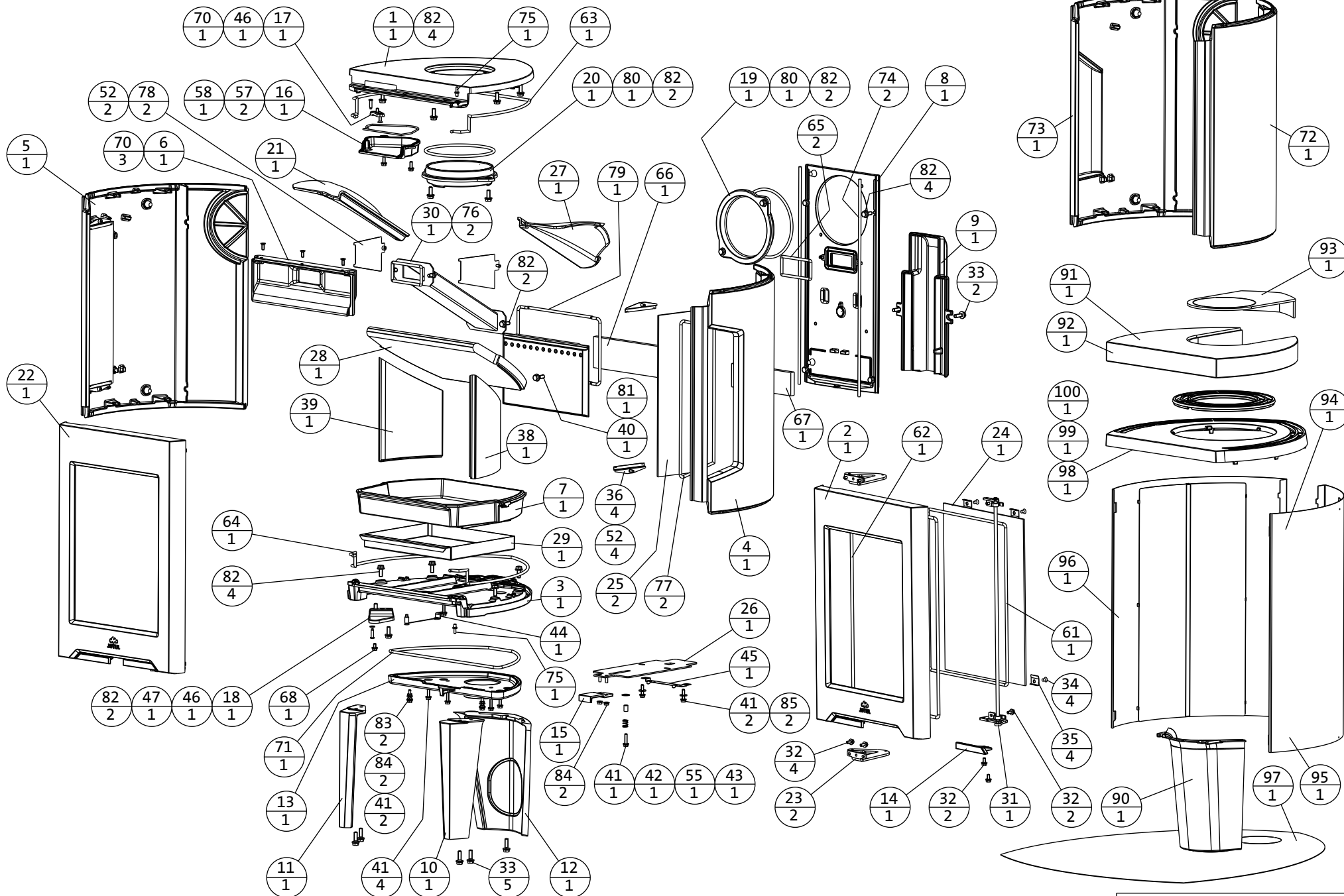
Exploded view Jøtul F 160 Jøtul AS Fredrikstad, Norway Drawing.no: 900049-Poz Date: Nov. 2010
